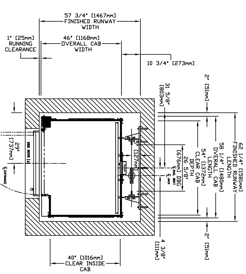
PLAN VIEW - INFINITY Model 4054 TYPE 5
