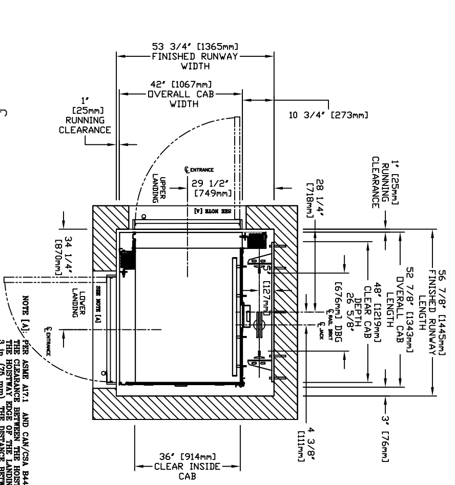
PLAN VIEW - INFINITY Model 3648 TYPE 4
