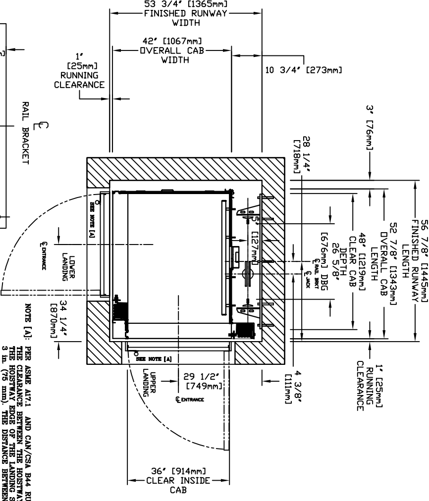
PLAN VIEW - INFINITY Model 3648 TYPE 3
